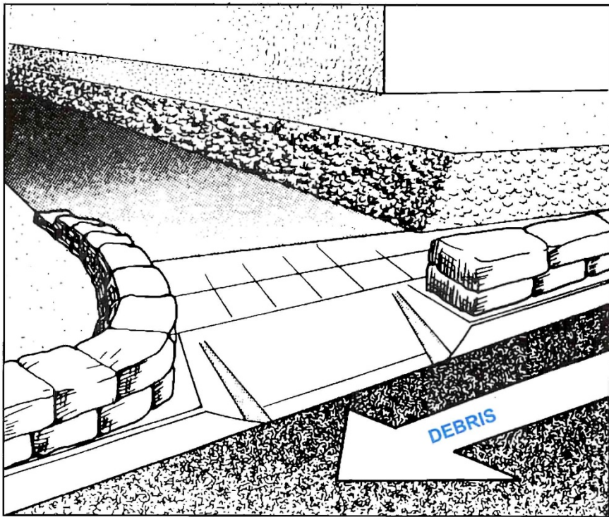
Fig. 8 CONTROLLING DEBRIS OR STORM FLOWS IN STREETS
