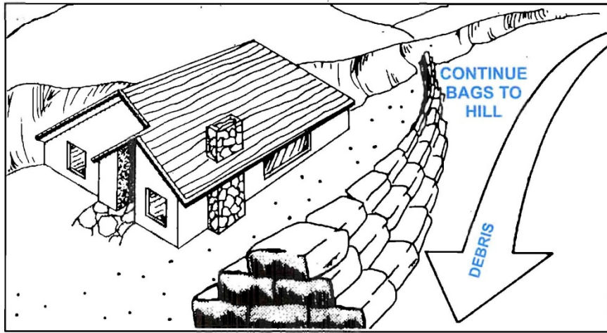
Fig. 7 DIRECTING DEBRIS AWAY FROM BUILDINGS
