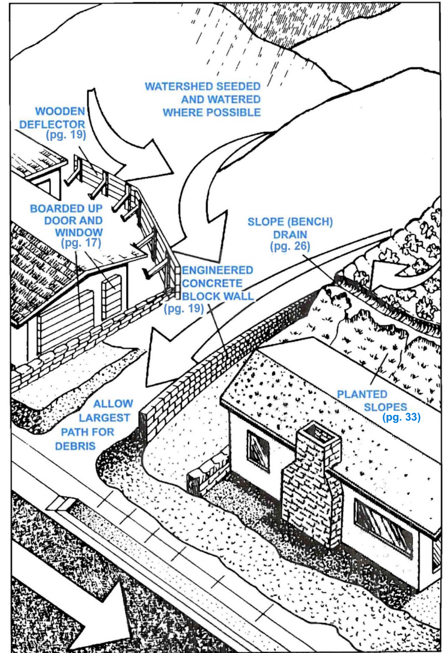
Fig. 2 HOMES PROTECTED FROM MAJOR DAMAGE
