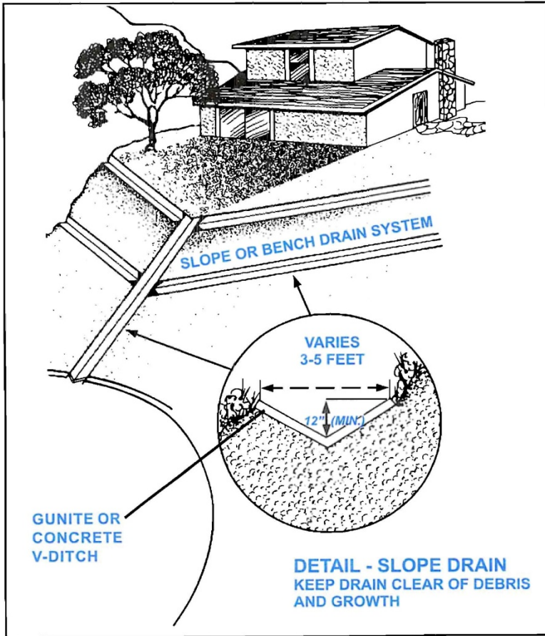
Fig. 22 SLOPE (BENCH) DRAIN
