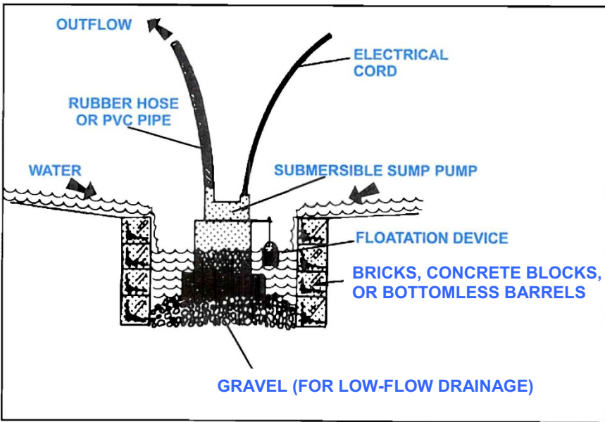
Fig. 13 SUBMERSIBLE SUMP PUMP
