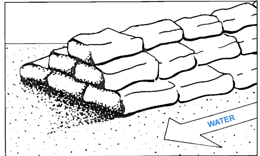
Fig. 6 PYRAMID SANDBAG STACKING
