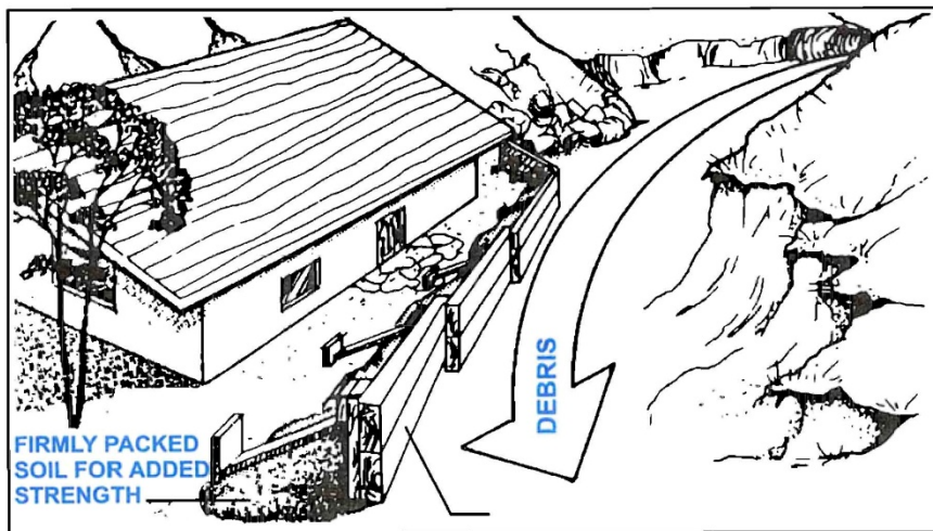
Fig. 17 TIMBER DEFLECTOR
