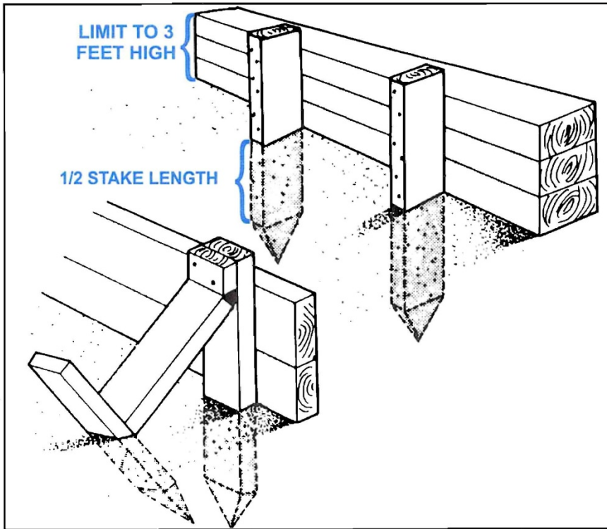
Fig. 16 TYPICAL TIMBER INSTALLATION
